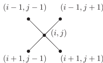
Figure 1. Neighbors of the vertex (i, j) .
