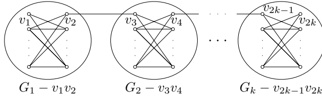
Figure 1. Bipartite graph: G_{\Delta, k} .
