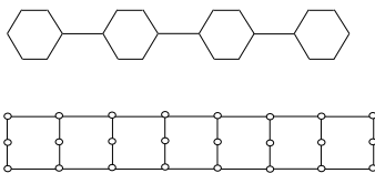
Figure 6: Two weakly elementary bipartite graphs in which every normal block is a cycle.
