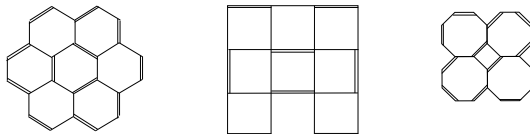
Figure 2: Some types of plane bipartite graphs that its interior vertices are of the same degree.
