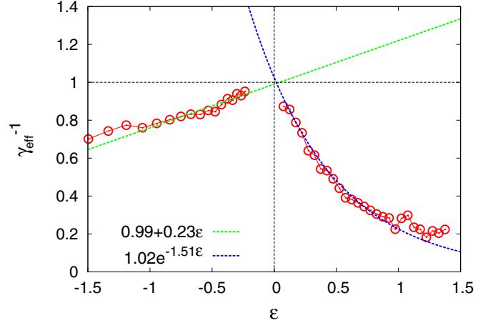
FIG. 4. (Color online) Numerical data for the inverse of the effective exponent \gamma_{\text{eff}}^{-1} are plotted against \epsilon for N = 12800 . Two dotted lines represent the fitting lines, indicating \gamma \approx 0.98 and \gamma' \approx 1.01 .
