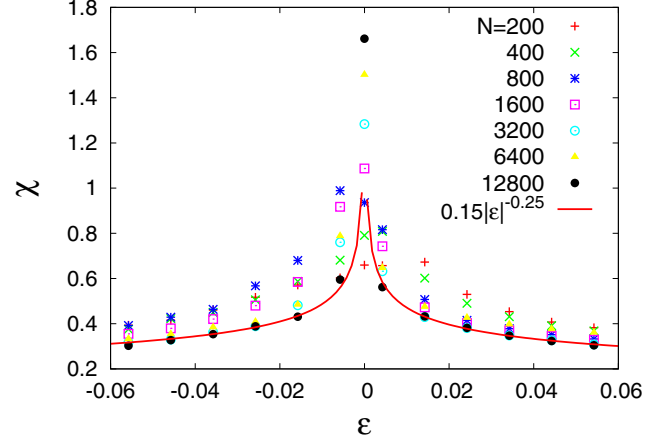
FIG. 8. (Color online) Dynamic fluctuation \chi is plotted as a function of \epsilon (=K - K_c) for various system sizes N for the regular distribution, where K_c = \sqrt{8/\pi} . The solid (red) line represents a fitting line for data with the largest system size.
