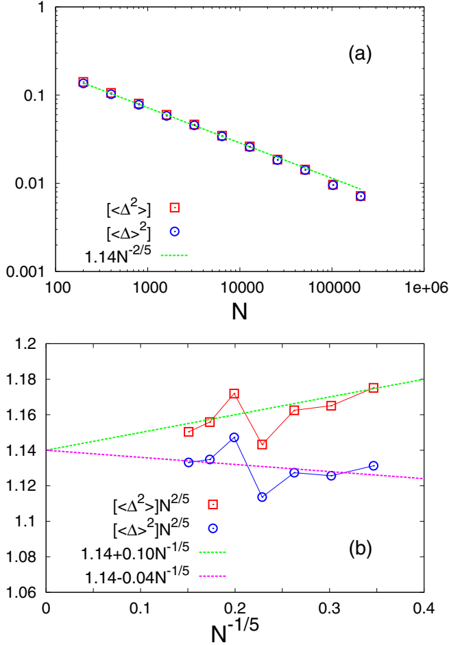
FIG. 5. (Color online) (a) Critical decay of [\langle \Delta^2 \rangle] and [\langle \Delta \rangle^2] at K_c ( =\sqrt{8/\pi} ) is plotted against N in a log-log plot. These two data are so close to each other that it is not possible to discern two data in this plot. The straight line is the fitting line of 1.14N^{-0.40} . (b) N^{2/5}[\langle \Delta^2 \rangle] and N^{2/5}[\langle \Delta \rangle^2] vs N^{-1/5} . These data are expected to show straight lines. The least-squares fitting yields two straight lines with the same intercept. Lines between data are only guides to the eye.
