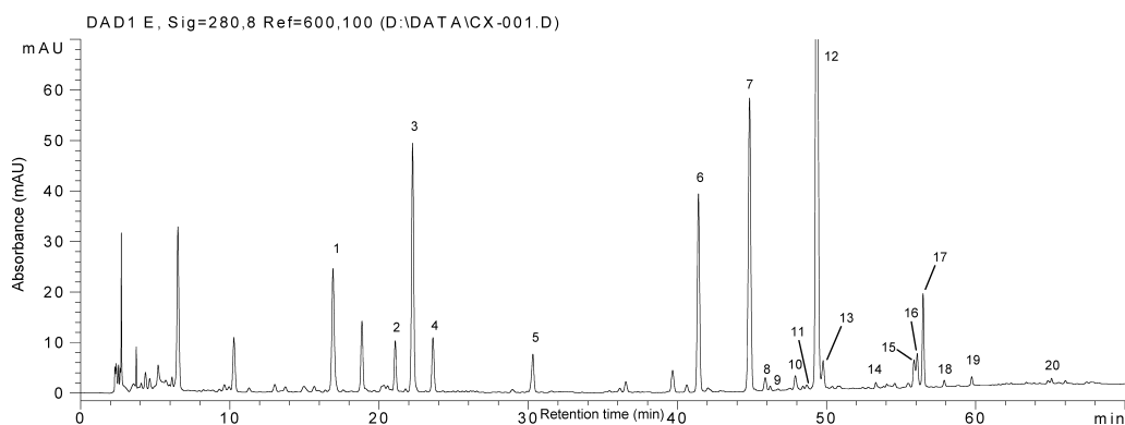
Fig. 1. Typical HPLC Chromatogram of Chuanxiong Samples at 280 nm
