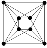
Figure 6.1: C_4 \circ K_2 .
