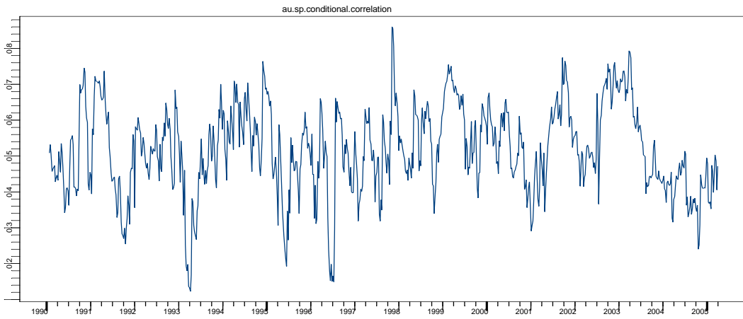
Figure 3. Conditional correlation between return series \Delta AU_t and \Delta SP_t
