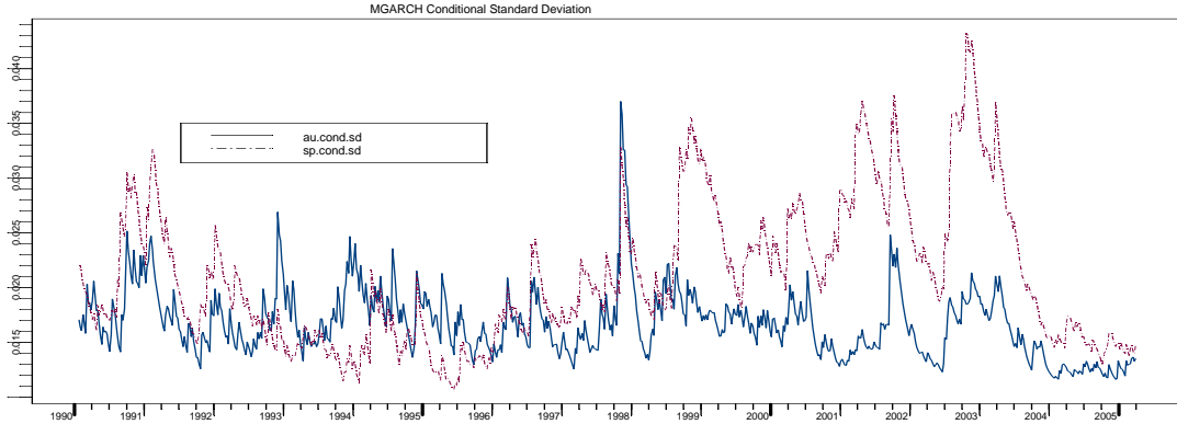
Figure 2. Conditional standard deviations for \Delta AU_t and \Delta SP_t
