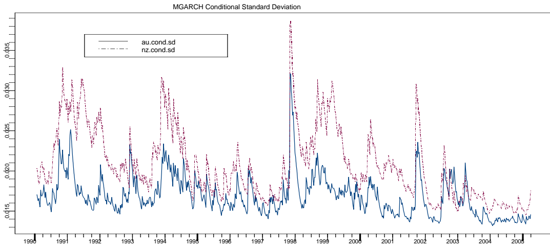
Figure 4. Conditional standard deviations for \Delta AU_t and \Delta NZ_t
