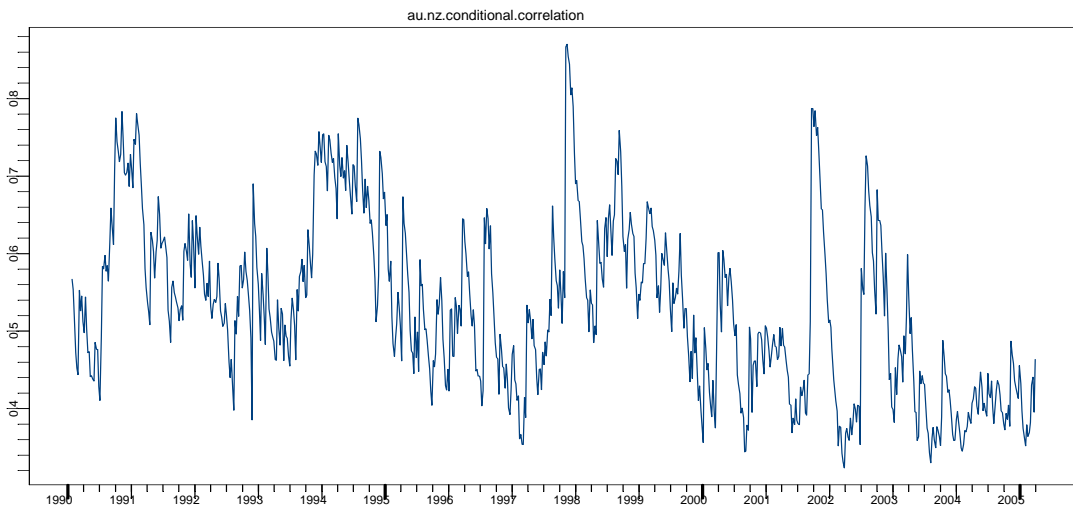
Figure 5. Conditional correlation between return series \Delta AU_t and \Delta NZ_t
