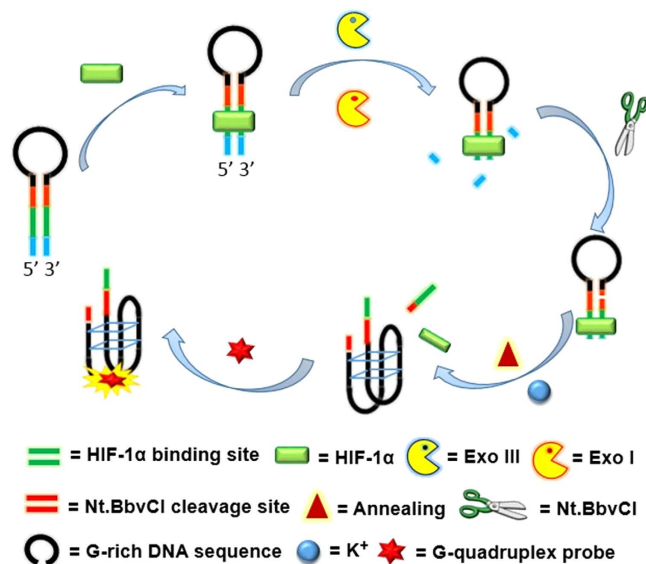
Figure 3. Schematic representation of the luminescent HIF-1α detection assay using a G-quadruplex probe.
